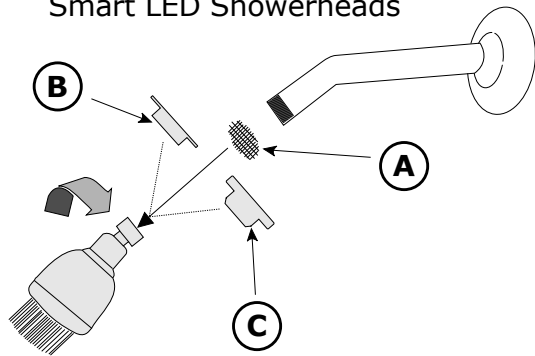
Flow Regulator
